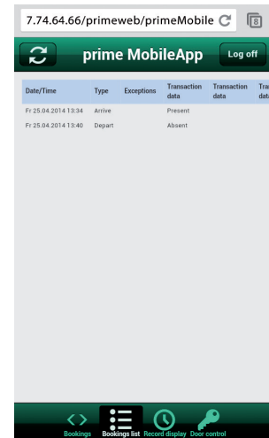
Bookings list
