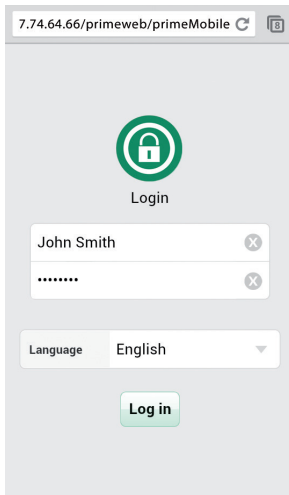
Login screen
