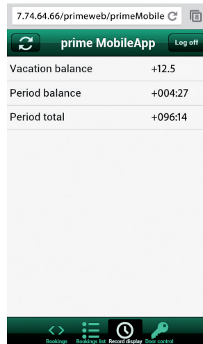
Record display
