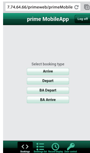
Booking types
