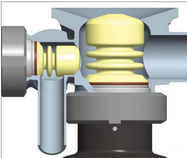
Sectional view of VESTA® Tank Bottom Valve with additional CIP/SIP valve
