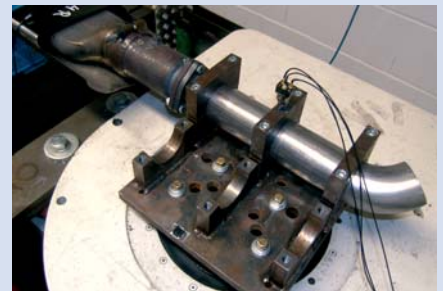
Manifold testing at ArvinMeritor Emissions Technologies GmbH in Augsburg/Germany
